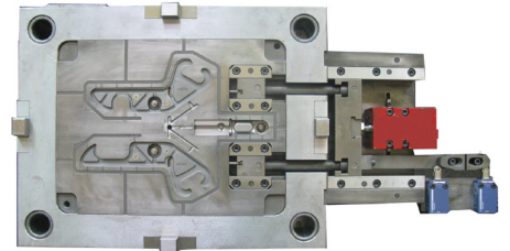
AM12885 450x400x331(mm)cav
