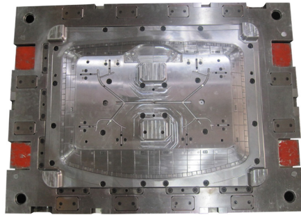
AM121015 990x1350x701(mm)core
