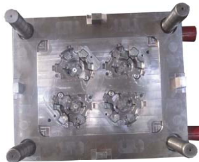
AM141491 550x550x654(mm)Core
