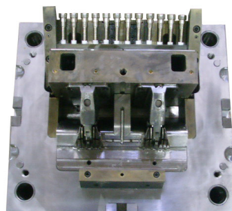
AM12971-2 560x560x642(mm)core
