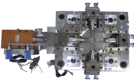
AM131081 318x400x371(mm)core
