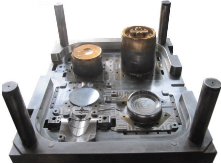
AM12909-2 1000x850x976(mm)core
