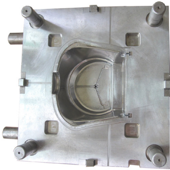
AM12869-1 500x530x501(mm)cav
