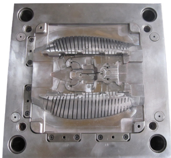
AM12946-2 576x590x467(mm)core
