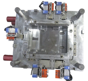
AM131088-2 600x700x592(mm)cav
