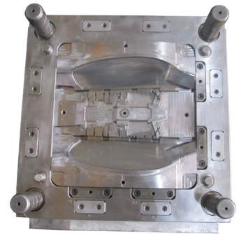
AM12946-1 576x590x467(mm)cav
