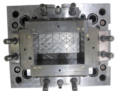
AM12993-1 520x650x635(mm)cav
