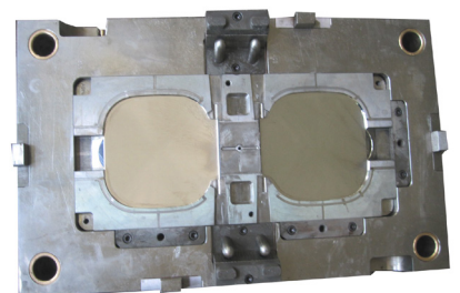
AM12867 450x750x406(mm)cav
