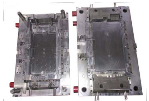
AM151716 1000X780X661(mm)
