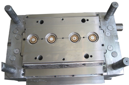
AM12896-1 500x350x481(mm)core
