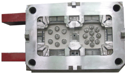
AM12890-1 320x400x412(mm)core
