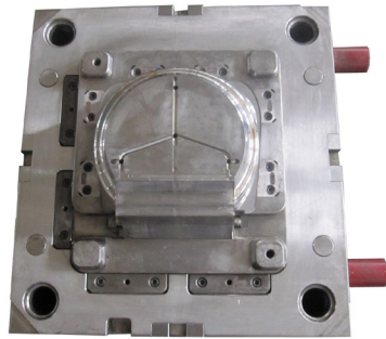
AM12920-2 530x595x501(mm)core
