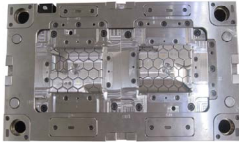
AM151656 600x400x572(mm)cav
