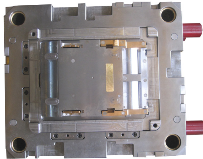
AM131088-1 600x700x592(mm)core
