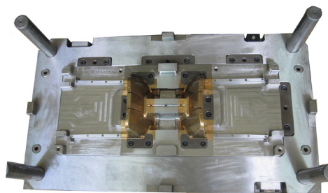
AM12864-1 450x800x556(mm)core
