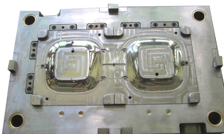
AM12866-1 450x700x406(mm)cav
