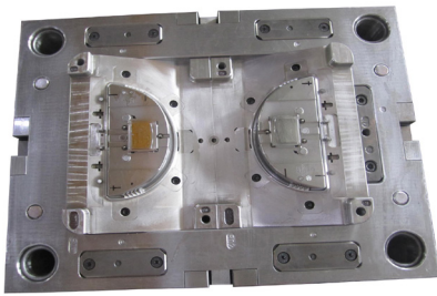
AM121022-2 400x450x391(mm)core
