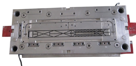
AM12899 350x750x351(mm)core
