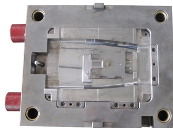
AM12966-1 450x550x490(mm)cav
