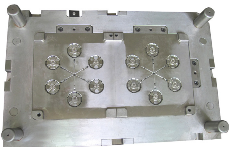
AM12891-2 500x900x526(mm)cav
