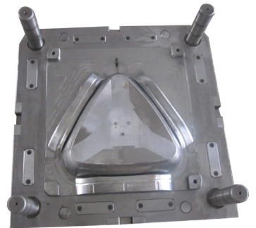
AM12840-1 600x600x638(mm)core
