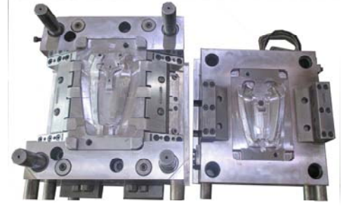
AM151655 530X500X600(mm)
