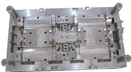
AM12891-2 500x900x526(mm)cav
