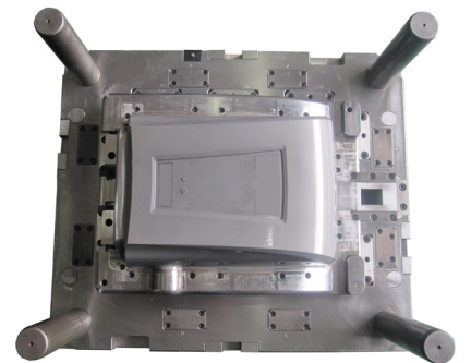
AM131190 600x700x621(mm)core
