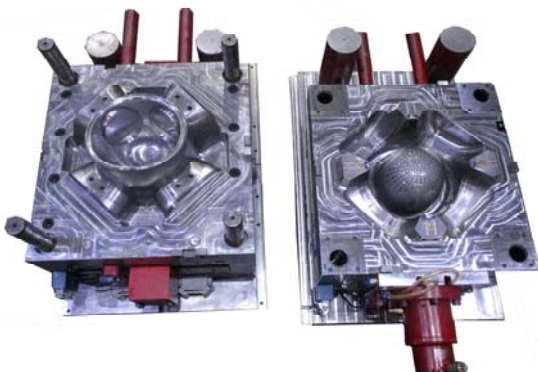
AM141486 1106x710x837(mm)
