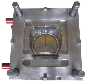
AM12920-1 530x595x501(mm)cav
