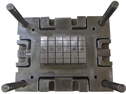
AM12993-2 520x650x536(mm)core
