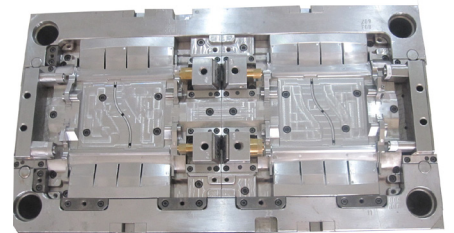
AM12891-1 500x900x526(mm)core
