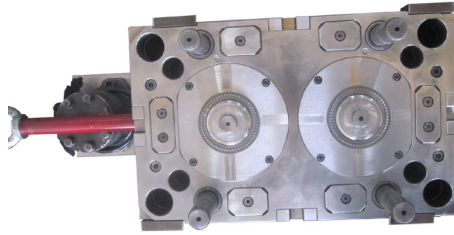
AM131041 300x400x526(mm)core
