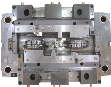
AM131185 450x700x506(mm)core
