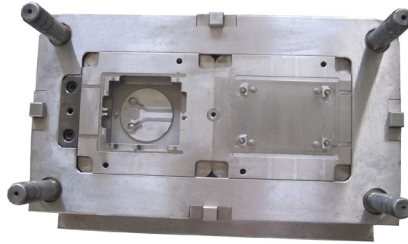
AM12912-1 450x320x341(mm)cav
