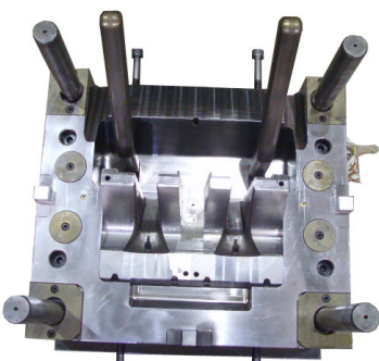
AM12971-1 560x560x642(mm)cav
