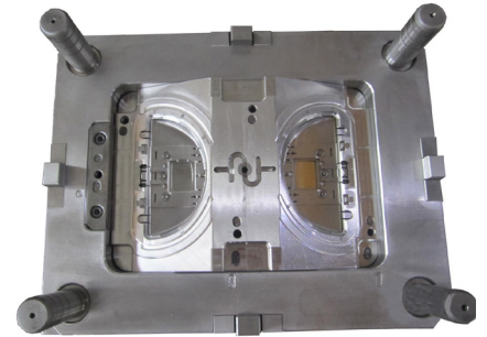
AM121022-1 400x450x391(mm)cav
