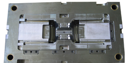
AM12864-2 450x800x556(mm)cav
