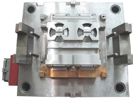
AM12877 500x550x546(mm)cav
