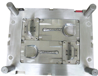
AM12863-1 597x750x656(mm)core
